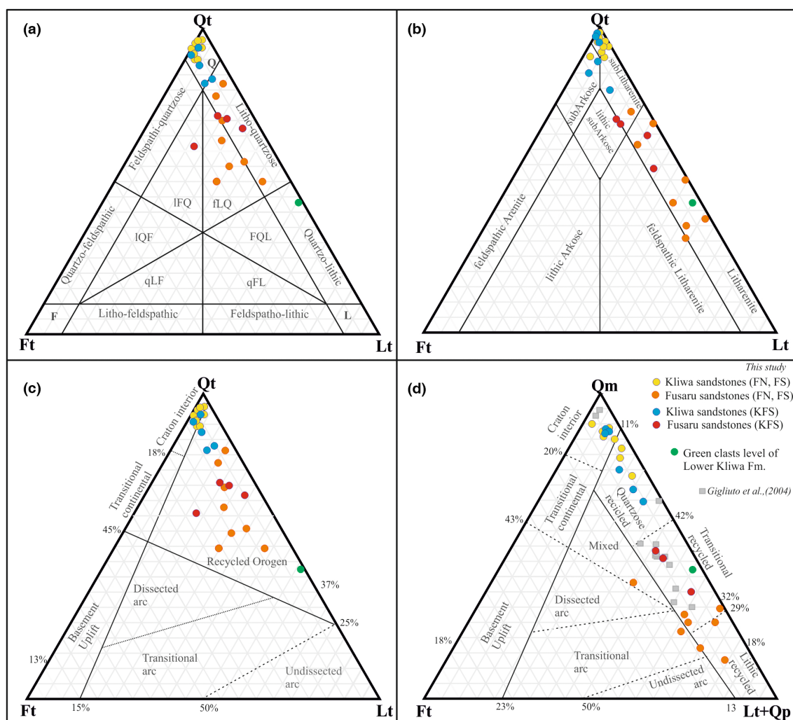
FIGURE 10 Petrographical data plots. (a) According to Garzanti (2019) classification, Kliwa sandstones are quartzose and Fusaru sandstones are lithic and feldspatho-litho quartzose; (b) The classical classifications (McBride, 1963) show that quartzose arenite and subordinate sub-feldspathic or sub-lithic arenite are typical for Kliwa samples while Fusaru sandstones are characterized by litharenite; (c) QtFtLt diagram of Dickinson (1985), shows the tectonic framework of an inner craton (Kliwa sandstones) and recycled orogen (Fusaru sandstones); (d) QmFt Lt + Qp diagram (Dickinson, 1985) suggests a craton interior and quartzose recycled orogenic fields: recycled quartzose for Kliwa sandstones and transitional to lithic recycled orogen fields for Fusaru sandstones.
