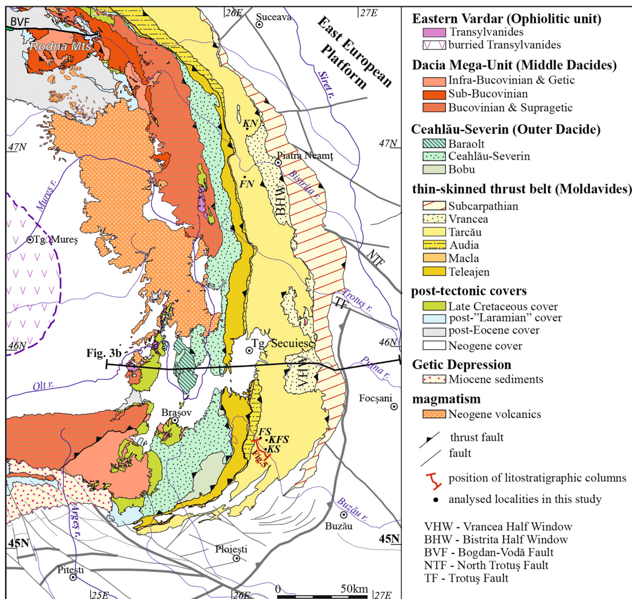
FIGURE 2 A detailed fragment of the tectonic map displayed in Figure 1b, focusing on the East Carpathians, after Geological Institute of Romania maps, Maţenco (2017) and references therein. The black line shows the location of the geological section from Figure 3b. The red line indicates the sections from Figure 5: FN (Fusaru North—Tarcău locality); KN (Kliwa North—Sihla locality); FS (Fusaru South—Siriu Dam Lake), KS (Kliwa South—Buzău Valley, Şeţu rail station) and KFS (Kliwa and Fusau South—Vineţişu locality) are the locations of the sections described in this study.
